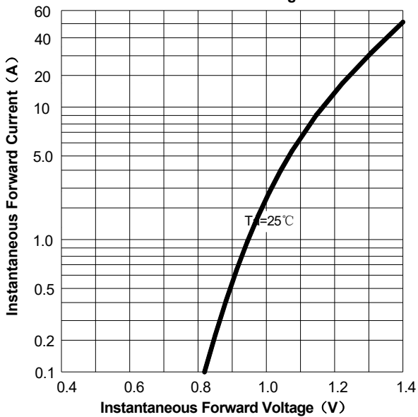
FIG3: Forward Voltage
