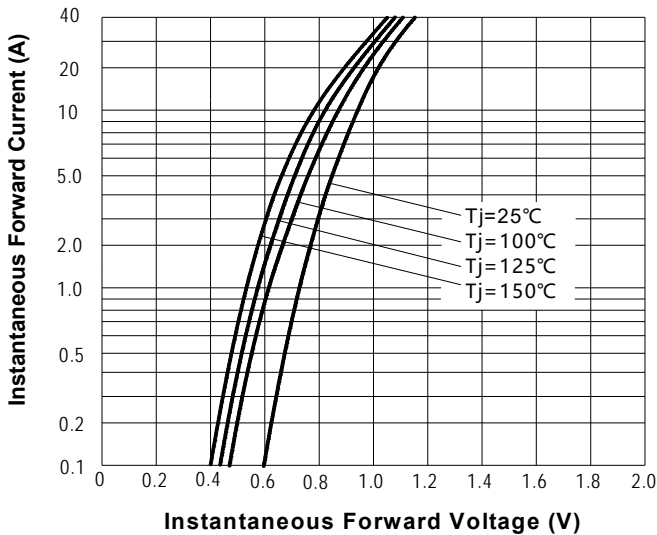
FIG3: Forward Voltage
