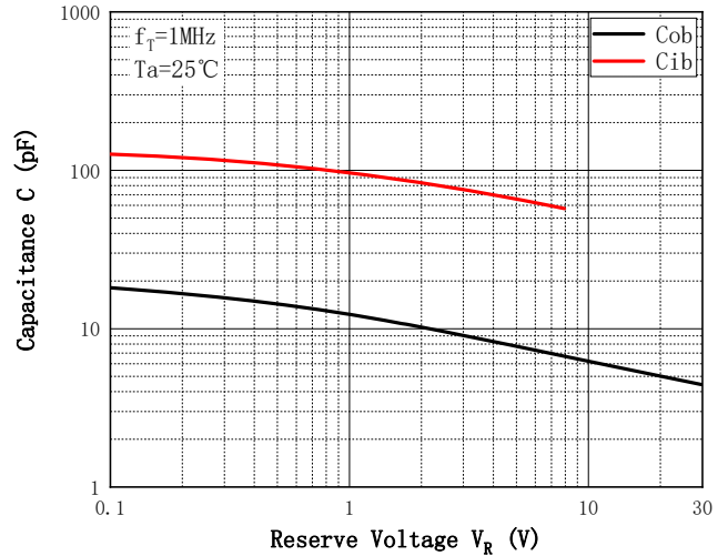
Fig. 6 - C_{ob}/C_{ib} - V_{CB}/V_{EB}
