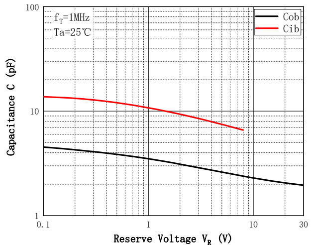
Fig.6 - C_{ob}/C_{ib}-V_{CB}/V_{EB}
