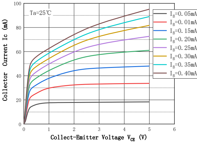
Fig.1-Static Characteristic
