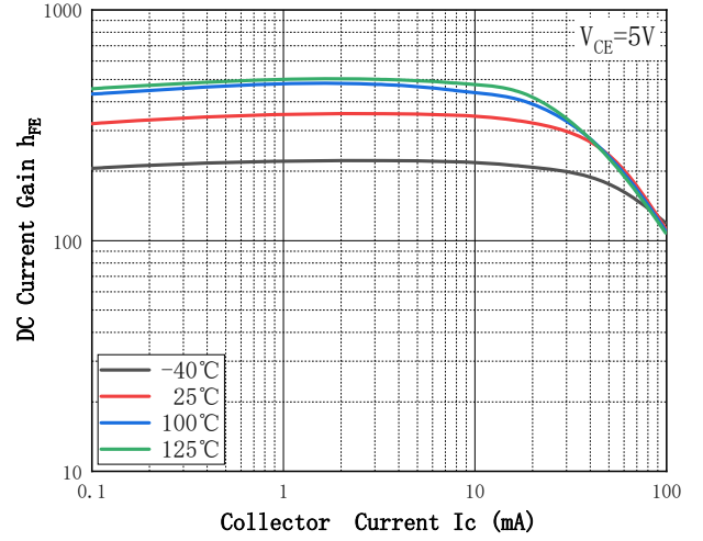
Fig.2 - DC Current Gian
